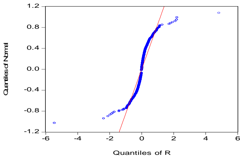
Plot 2. Quantile-quantile plot of R(t) distribution against Gaussian PDF with the same mean and standard deviation
