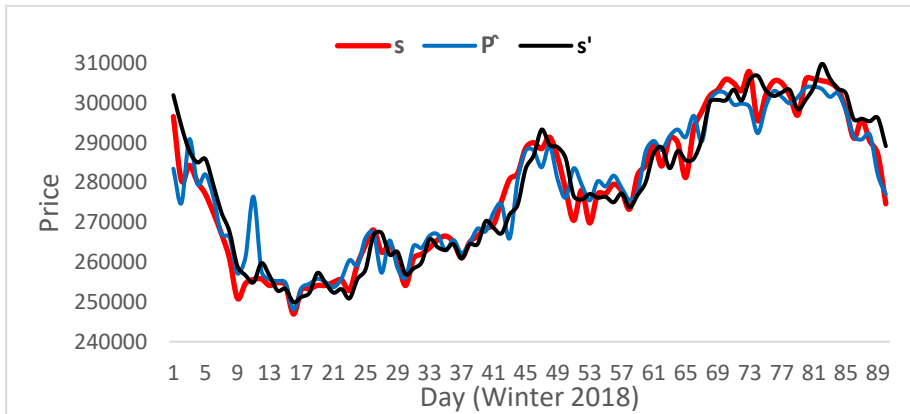
Figure 12. Actual ( s_t ) and fitted values of Price in Wavelet-ARMA-GARCH ( \hat{P}_t ) and ARIMA-GARCH ( s'_t ) Source: Research findings
