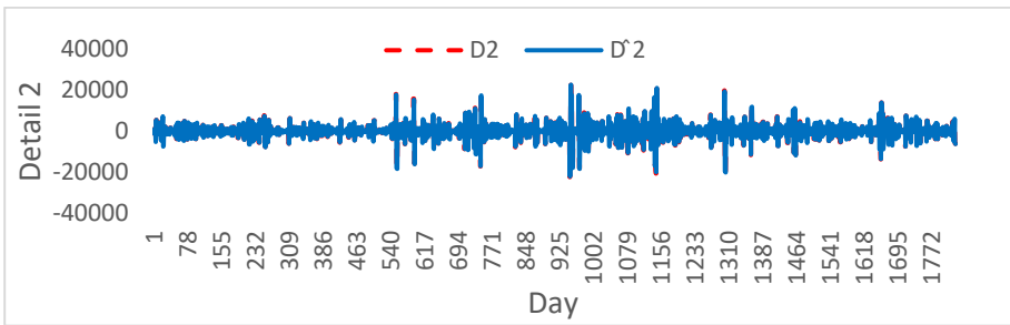
Figure 6. Actual and fitted values of D2 ( D2_t & \widehat{D2}_t )
