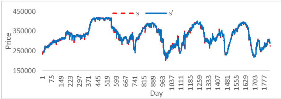
Figure 10. Actual and fitted values of Price( s_t & s'_t )
