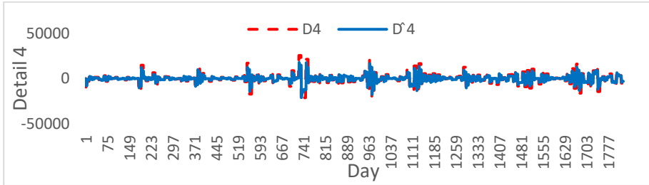
Figure 8. Actual and fitted values of D4 (D4_t \& \widehat{D4}_t) Source: Research findings
