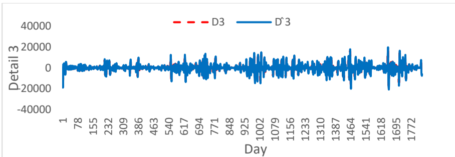
Figure 7. Actual and fitted values of D3 ( D3_t & \widehat{D3}_t )
