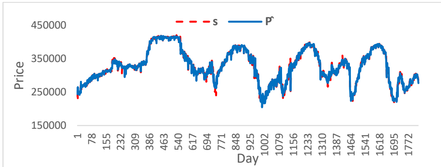
Figure 9. Actual and fitted values of Price ( s_t & \hat{P}_t ) Source: Research findings
