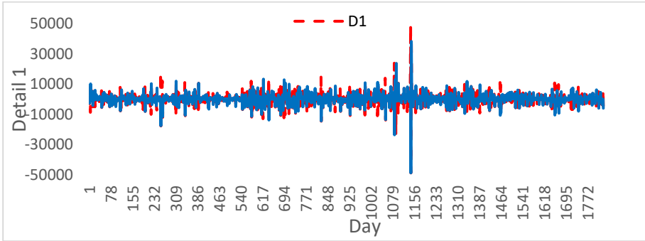
Figure 5. Actual and fitted values of D1 ( D1_t & \widehat{D1}_t )
